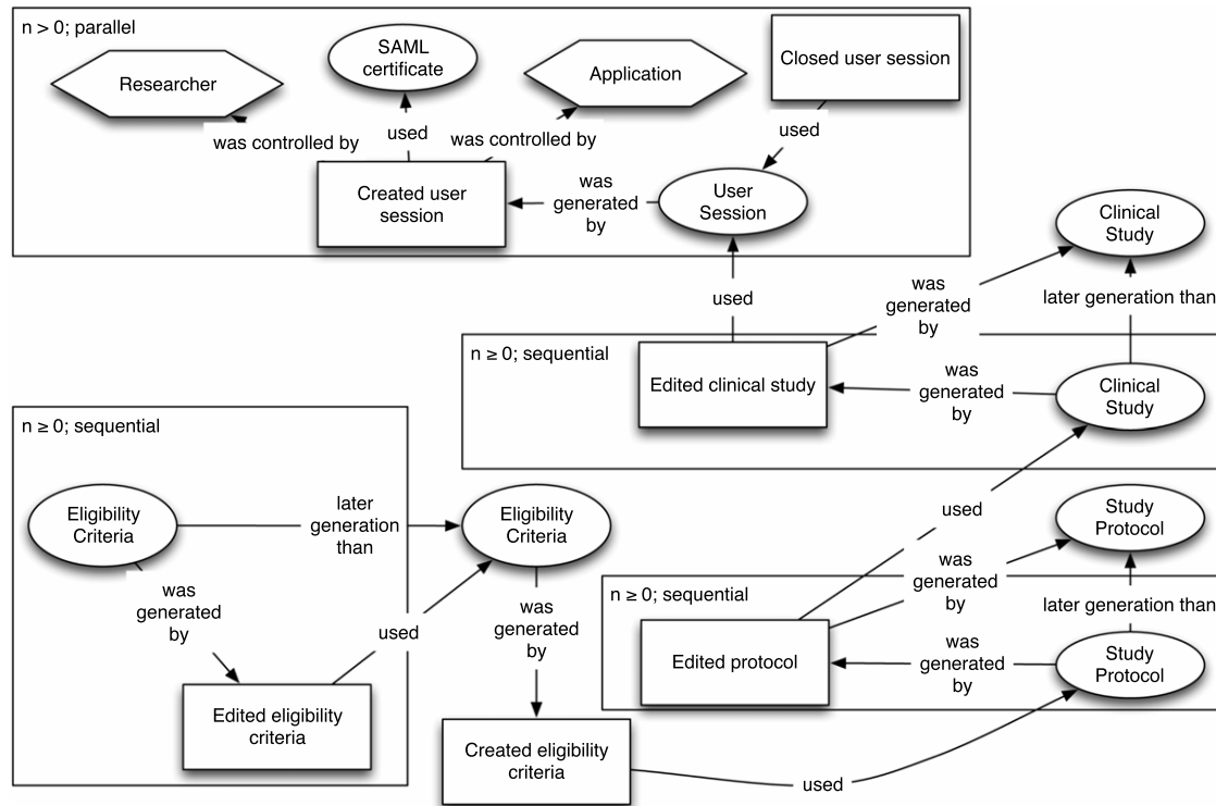
Fig. 2. A TRANSFoRm provenance template taken from Query Formulation Tool, describing creation and editing of eligibility criteria, as specified in the CRIM model.
