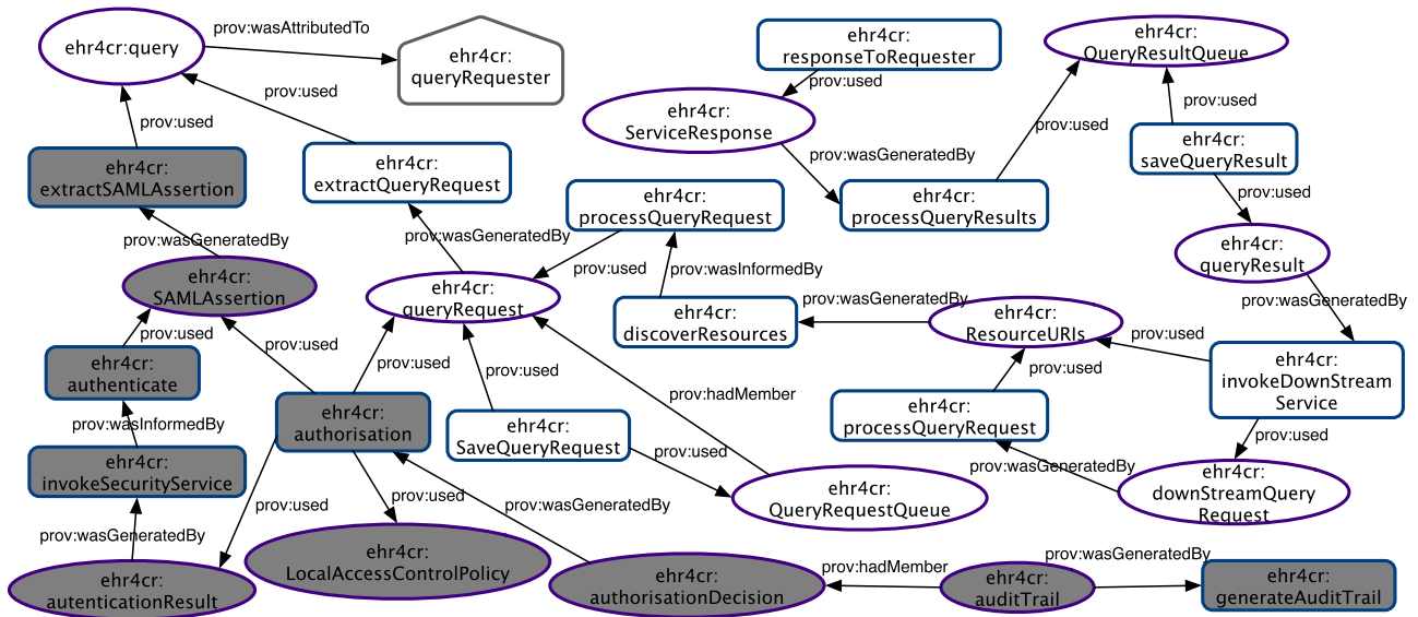
Fig. 5. A provenance recording template for integrated auditing.
