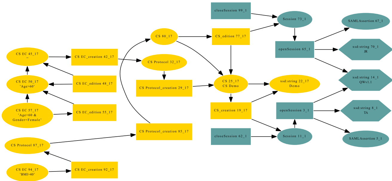
Fig. 3. Provenance graph conforming to the template in Fig. 2 contains the trace of the evolution of a clinical study entity 'CS Demo' during the study preparation phase. Two versions of the entity are shown in the graph: 25_17 and 80_17, each one defining a protocol along with its eligibility criteria. Both versions were created using the same software tool, TRANSFoRm Query Workbench v1.1 (agent 14_1 in the graph) during two editing sessions opened by two different users (JR and TA). First version, 25_17, had a protocol created with eligibility criteria, initially empty (CS EC 45_17) and then edited twice to specify recruitment condition Age > 60 and Gender = Female. Another protocol (87_17) was created with eligibility criteria BMI > 40 and resulted in the new version of clinical study (CS 80_17). NB: CS and EC are label acronyms for ontological concepts in clinical study and eligibility criteria in RCTPO, colours denote different software tools that contributed different graph fragments, yellow for Query Workbench, blue for Authentication Framework. (For interpretation of the references to colour in this figure legend, the reader is referred to the web version of this article.)
