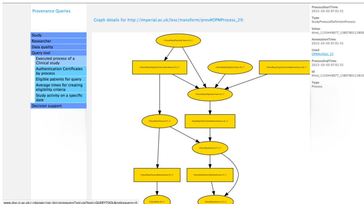
Fig. 4. TRANSFoRm query tool showing the graph area surrounding a selected item—StudyProtocolDefinitionProcess. The menu bar on the left contains configured queries.
