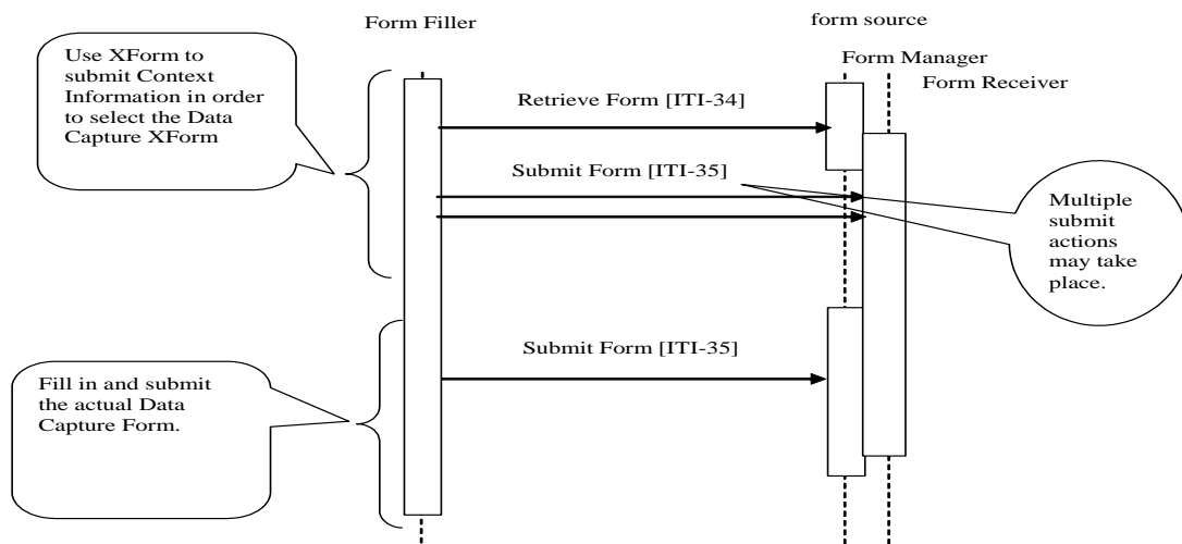
720 Figure 17.4-4 Case 4: Retrieve Form using an XForm; Submit Form
